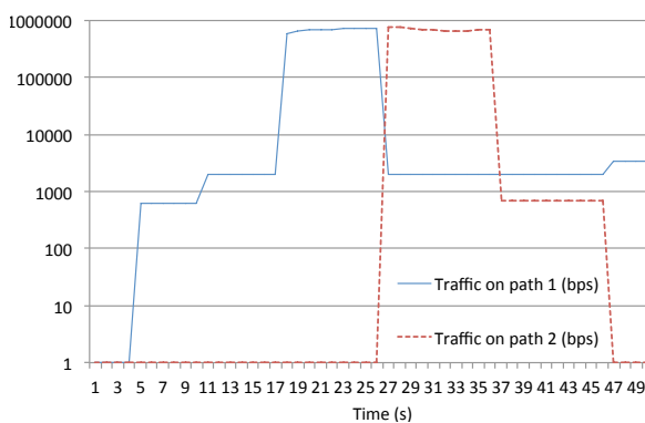
Figure 6.10: Detection of a large flow. When sender C starts a large flow, the controller tags it as elephant. Next it removes the tag when the load is reduced.
