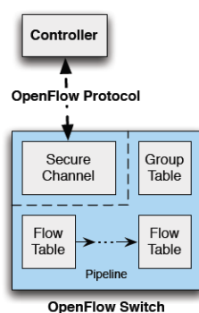
Figure 2.4: Components of an OpenFlow 1.1.0 switch. Source: [1].
