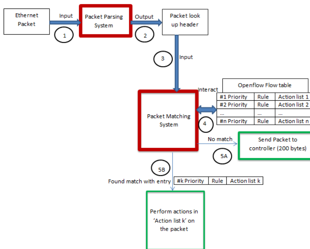
Figure 2.3: How a packet is processed and forwarded in an OpenFlow 1.0.0 switch.
