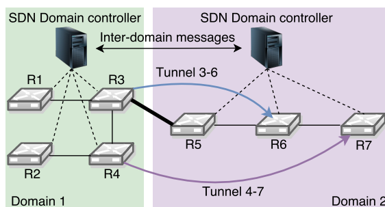
Figure 6.1: Sample network with two domains and two cut-through tunnels (3-6 and 4-7).
