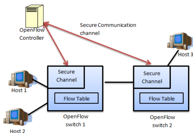
Figure 2.1: OpenFlow components.
