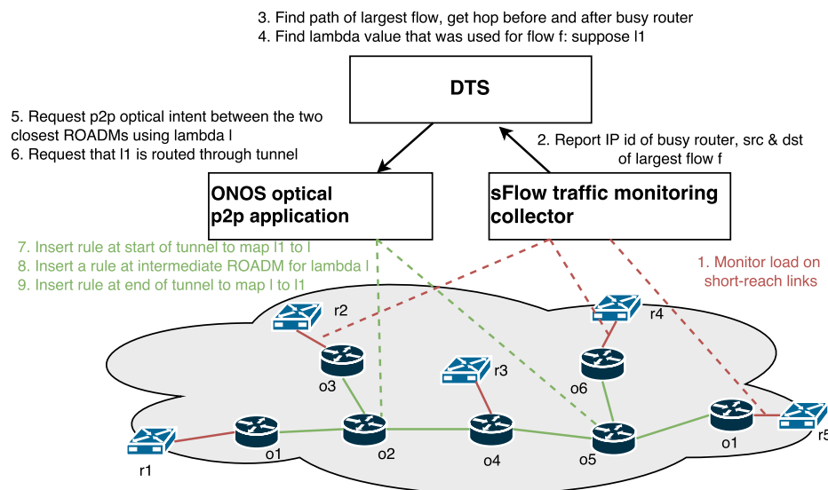
Figure 4.3: Operation of DTS using sFlow and a point-to-point optical intent application on ONOS
